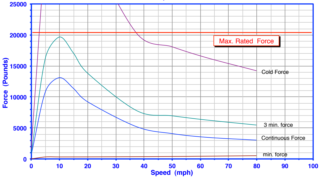
RS-90K Drawbar Pull 11.00 24.5 Tires, and 5.13:1 Drive Ratio
