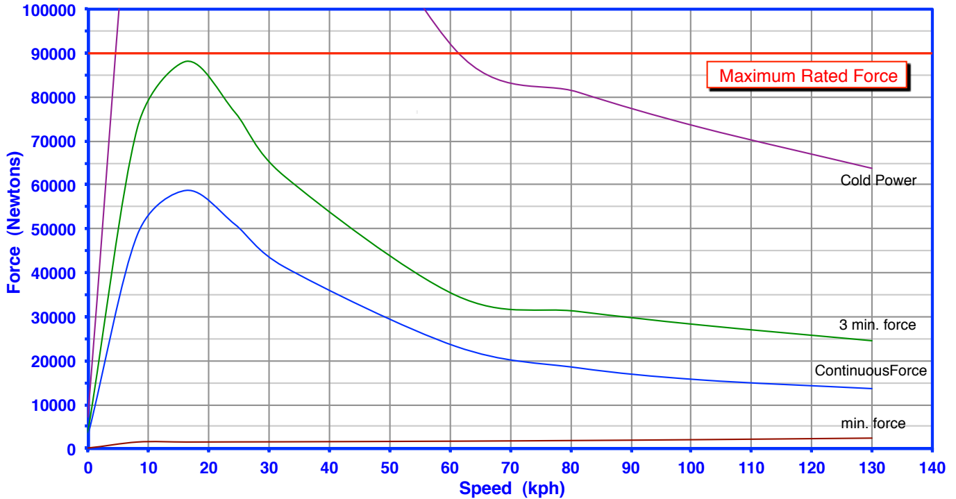
RS-90K Drawbar Force 11.00 24.5 Tires and 5.13:1 Drive Ratio
